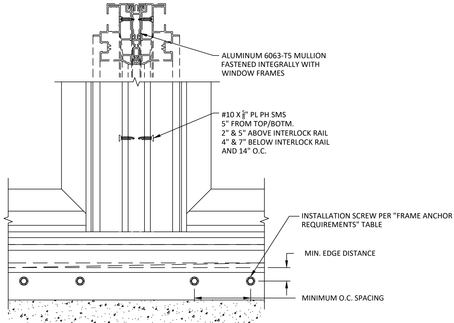
B 2 VERTICAL SECTION UNCLIPPED MULLION
