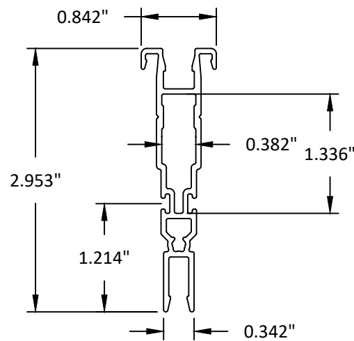
MULLION DETAIL
