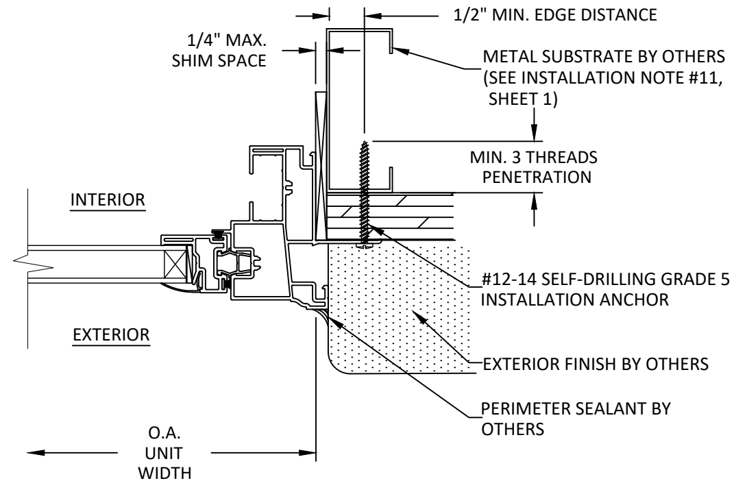
C 3 JAMB SECTION NAIL FIN INSTALLATION (HEAD & SILL ARE INSTALLED THE SAME)
