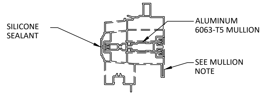
B 2 VERTICAL SECTION UNCLIPPED MULLION
